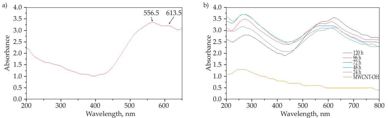
Fig. 2. UV-Vis spectra of the nanocomposites obtained at different reaction time: a) P3HT and b) P3HT/MWCNT-OH nanocomposites
