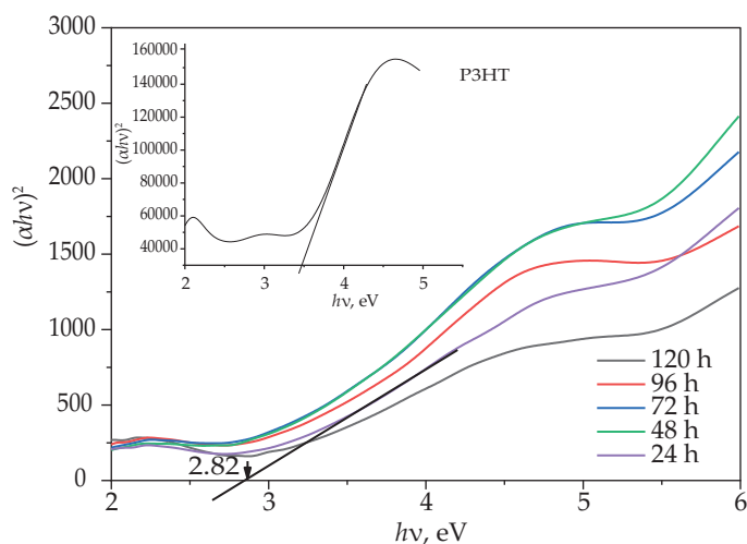
Fig. 3. Energy band gap of the P3HT and P3HT/MWCNT-OH nanocomposites obtained at different reaction time
