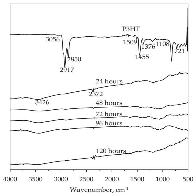
Fig. 1. FTIR spectra of the P3HT and P3HT/MWCNT-OH nanocomposite obtained at different reaction time
