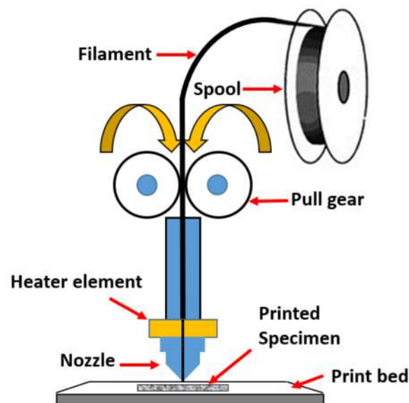
Figure 1. Schematic of a FDM 3D printing.
