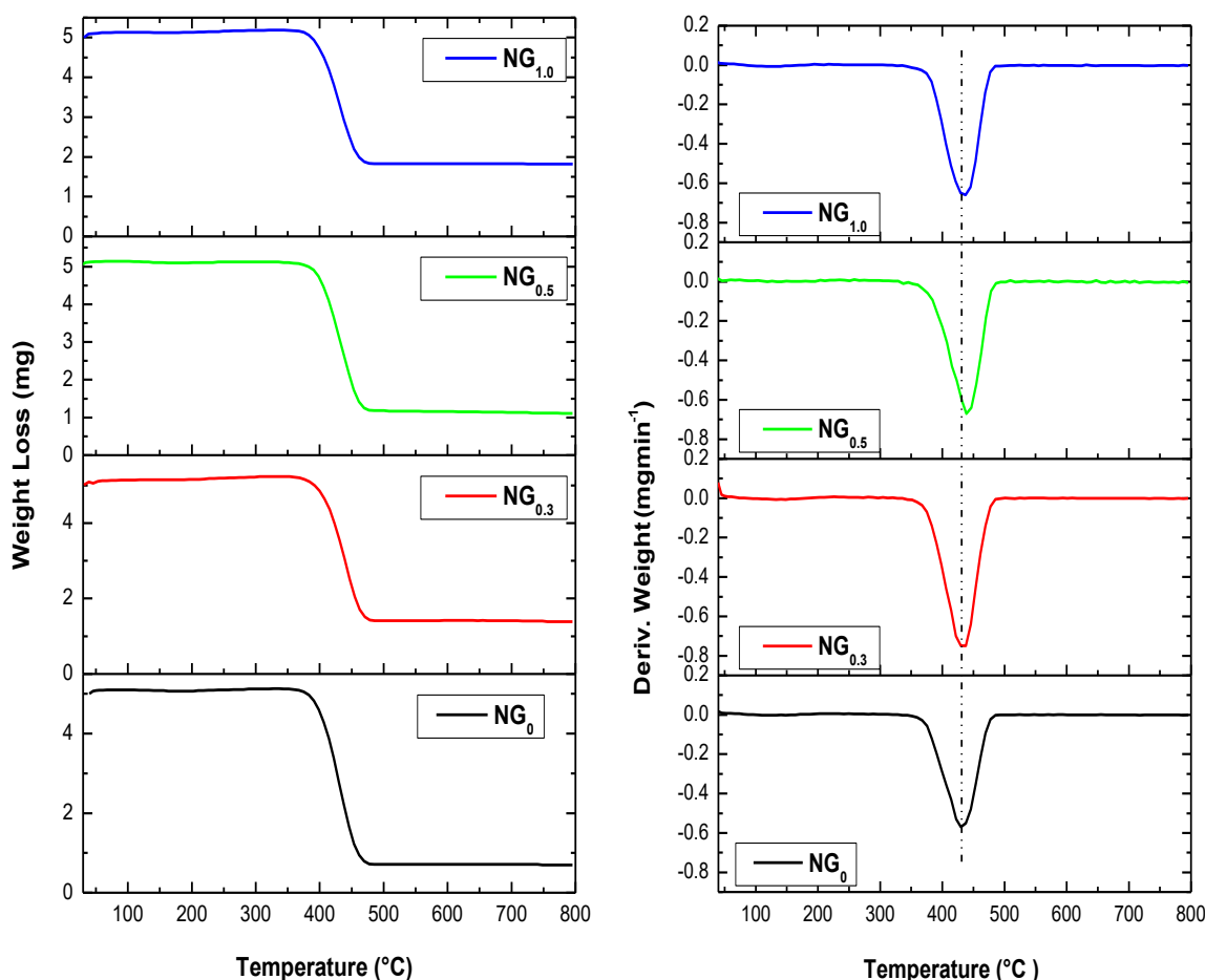
Fig. 3. (a) Thermogravimetric and (b) derivative thermogravimetric curves of nylon 66 and graphene nanoplatelet/nylon 66 nanocomposites
