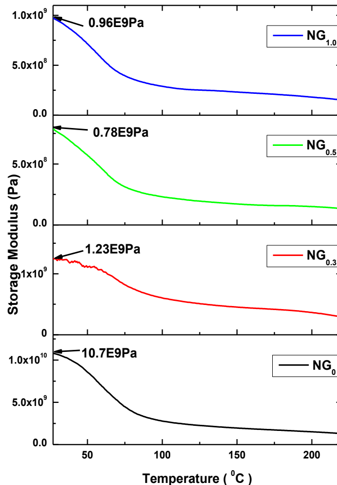
Fig. 5. Effect of GNP addition on the storage modulus of nylon 66/GNP nanocomposites
