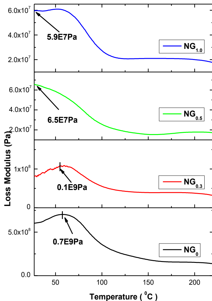
Fig. 6. Effect of GNP addition on the loss modulus of nylon 66/GNP nanocomposites
