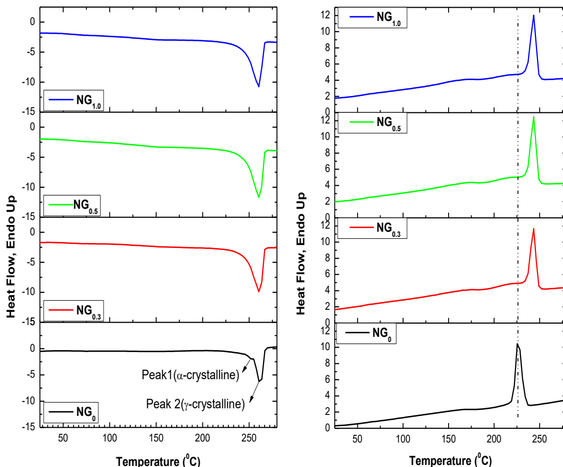
Fig. 2. (a) DSC thermograms of nylon 66/GNP during second heating and (b) DSC thermograms of nylon 66/GNP during cooling
