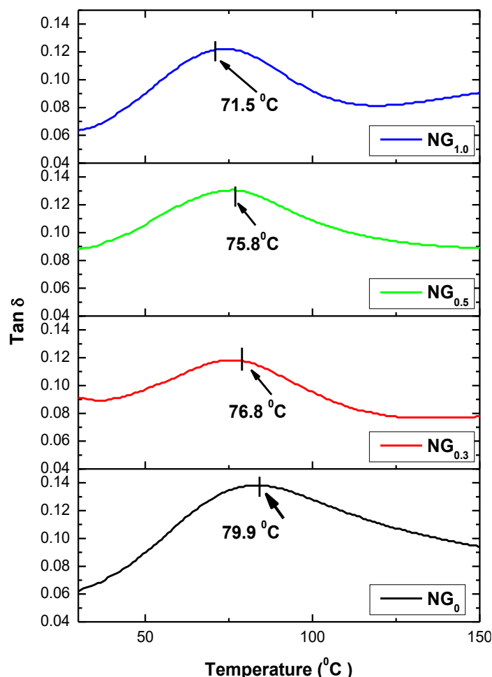
Fig. 4. Loading Effect on the \tan \delta of nylon 66 filled with various GNP amounts
