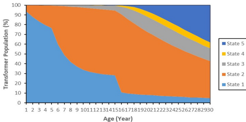
Figure 2. Transformer population distribution in each of the states with a 10% pre-determined maintenance repair rate performed at state 2
