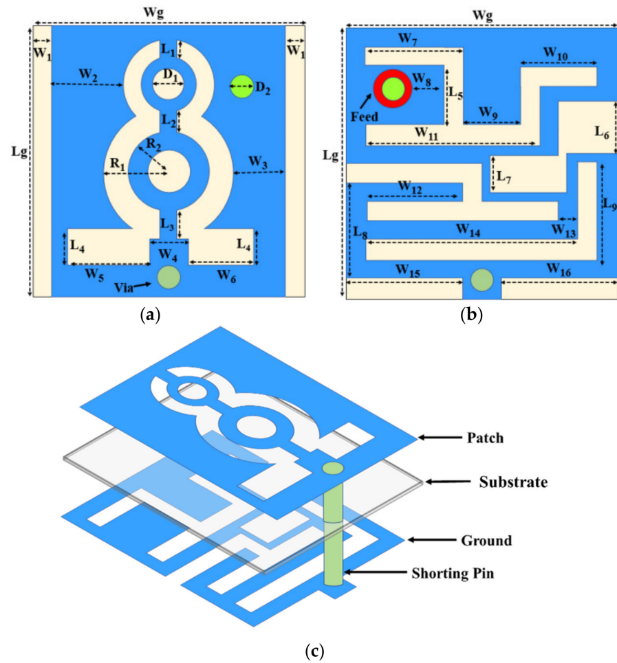
Figure 2. Stated design structure; (a) front view, (b) back view, and (c) 3D view.
