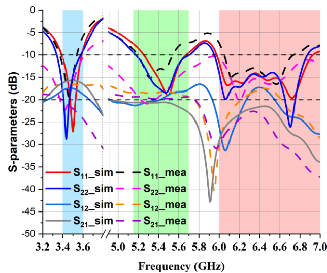
Figure 10. S-parameters ( S_{11} and S_{12} ) of the presented two-element MIMO antenna.
