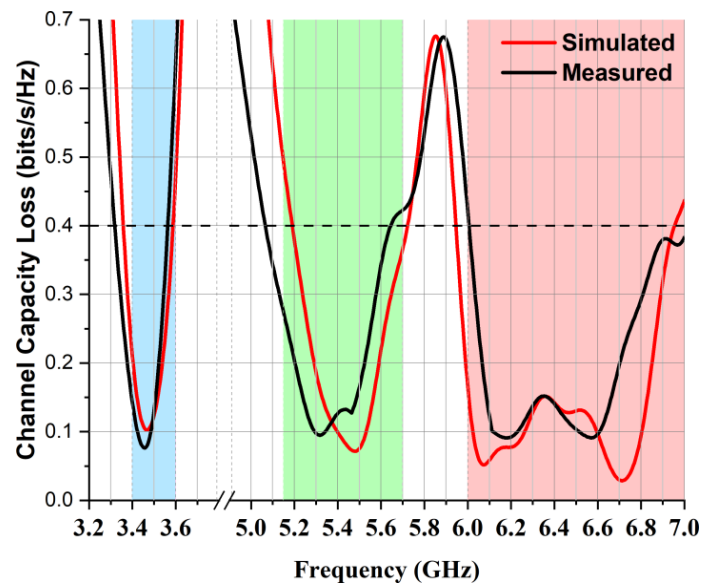
Figure 17. Channel capacity loss (CCL) of proposed two-element MIMO multiband antenna.
