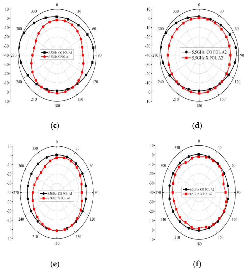
Figure 13. Co- and cross-polarization: (a) 3.5 GHz, Antenna 1; (b) 3.5 GHz, Antenna 2; (c) 5.5 GHz, Antenna 1; (d) 5.5 GHz, Antenna 2; (e) 6.5 GHz, Antenna 1; (f) 6.5 GHz, Antenna 2.
