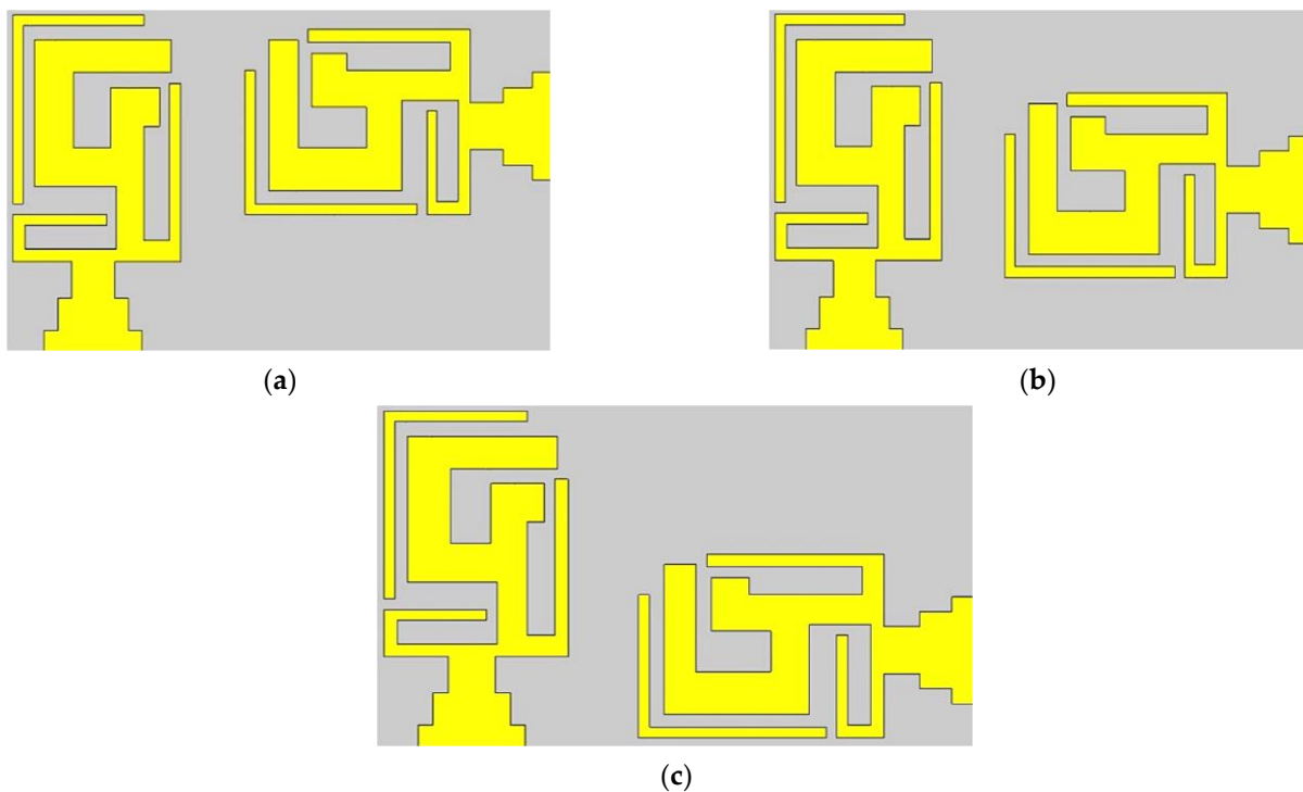
Figure 6. Different configurations of the two-element MIMO multiband antenna. (a) Top arrangement, (b) center arrangement, and (c) bottom arrangement.
