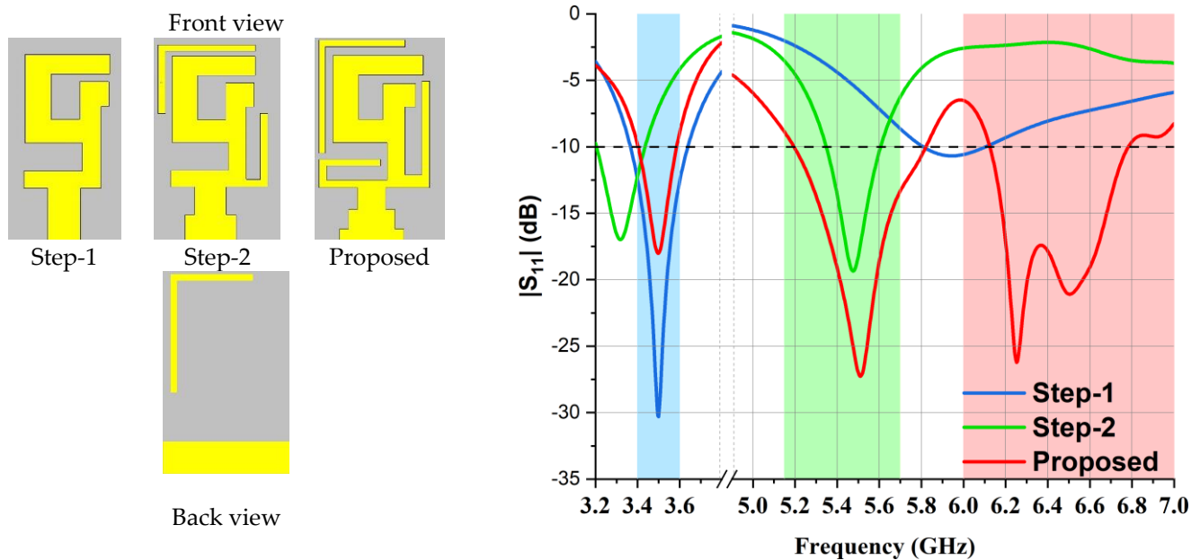
Figure 2. Simulated S_{11} results and design steps of single-element antenna.
