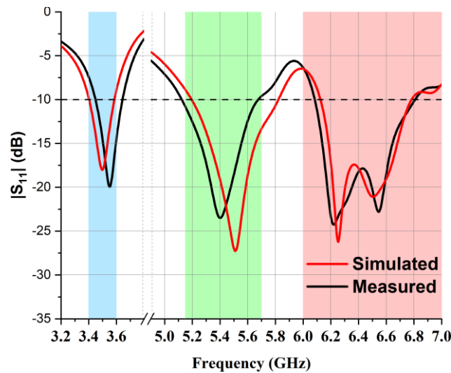
Figure 4. Laboratory-measured and simulated S_{11} of the single-element antenna.
