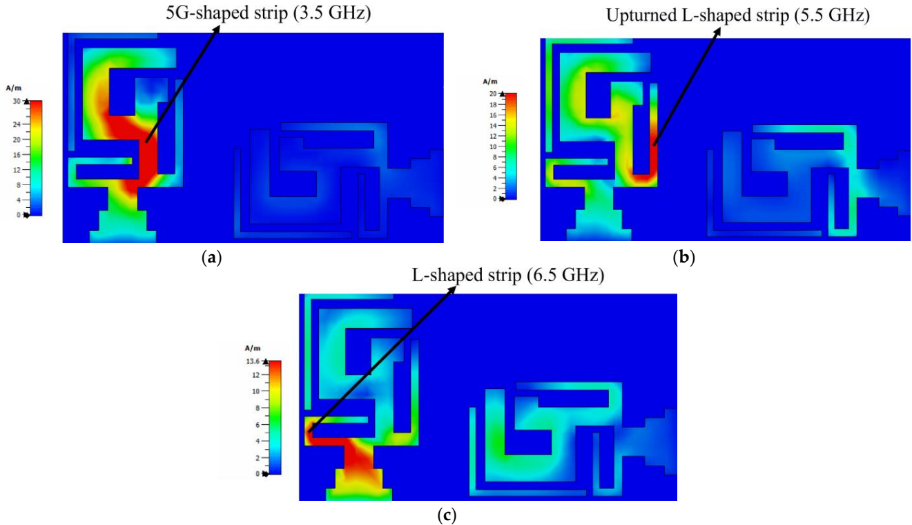
Figure 9. Current density of two-element MIMO multiband antenna: (a) 3.50 GHz, (b) 5.50 GHz, and (c) 6.50 GHz.
