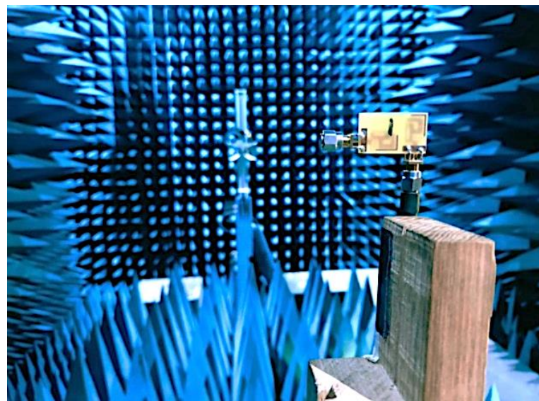
Figure 11. MIMO antenna anechoic chamber setup.
