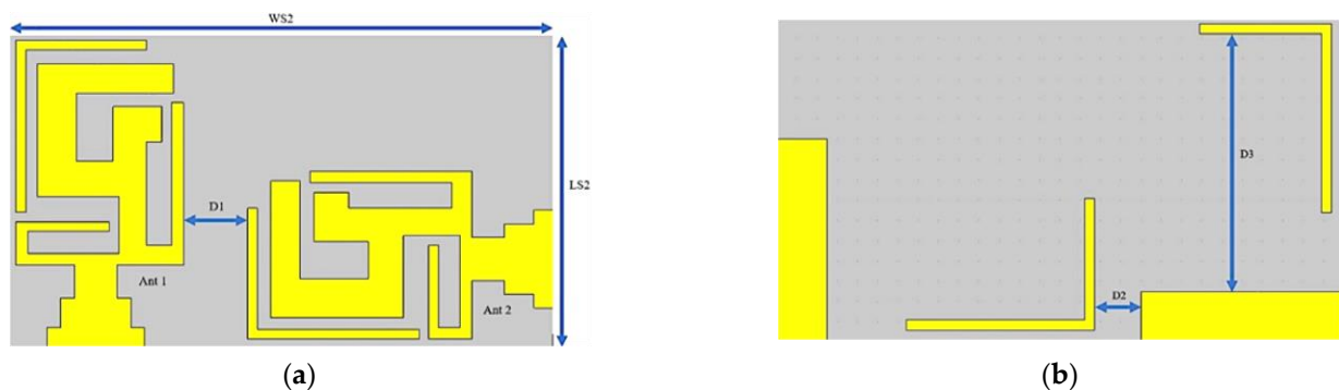
Figure 5. Two-element MIMO multiband antenna. (a) Top view and (b) bottom view.
