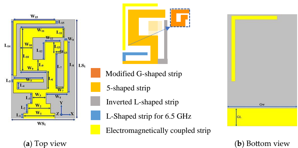
Figure 1. Top and bottom illustration of the single antenna element.
