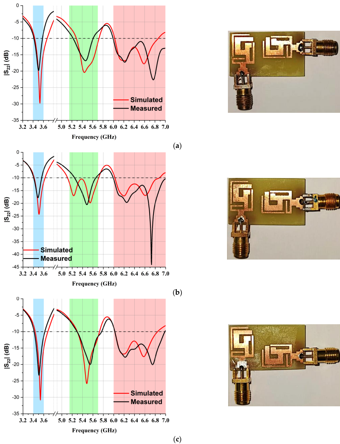
Figure 8. Comparison of reflection co-efficient ( S_{22} dB) at three different positions: (a) top position, (b) center position, and (c) bottom position.
