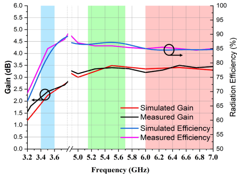
Figure 14. Radiation efficiency and gain of two-element MIMO multiband antenna.
