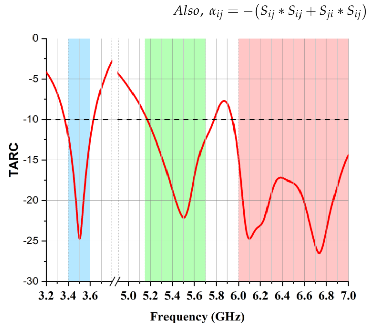
Figure 16. TARC of proposed two-element MIMO multiband antenna.
