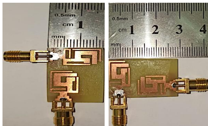
Figure 7. Fabricated design of two-element MIMO antenna.
