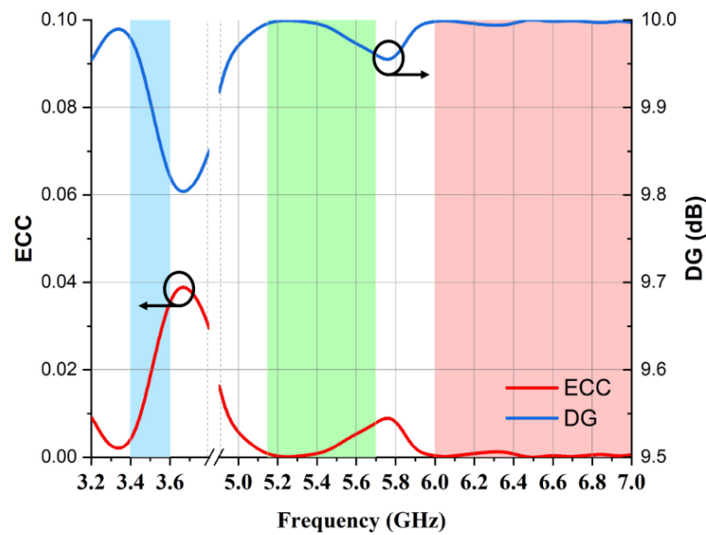
Figure 15. Calculated ECC and DG.
