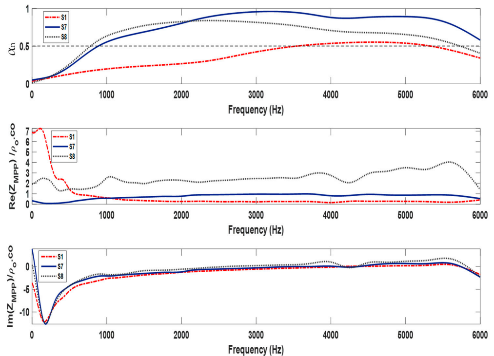
Figure 10. Sound absorption, resistive part, and reactive part of \tilde{Z}_{MPP} for woven fabric S1, S7, and S8.
