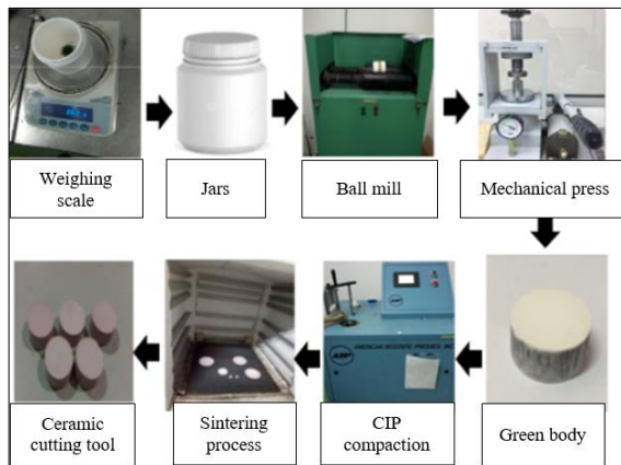
Figure 1: Process cutting tool development
