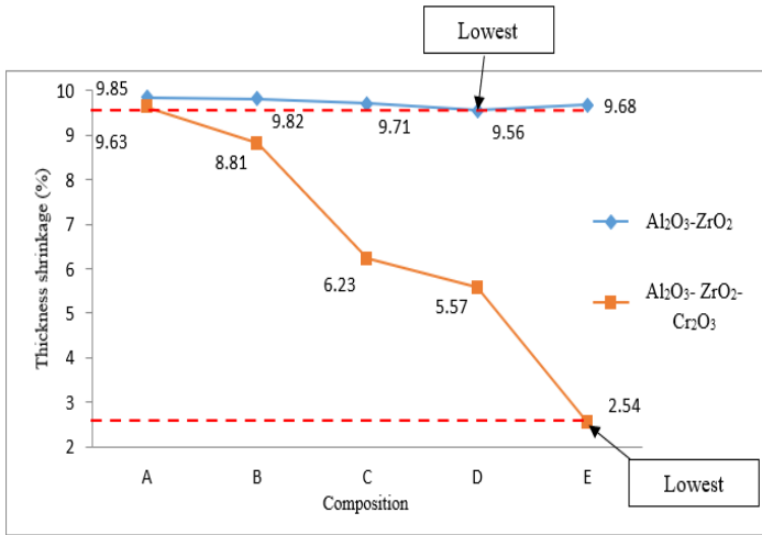
Figure 13: Comparison of thickness shrinkage in millimeters (mm)
