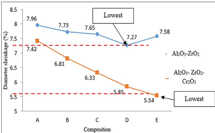
Figure 12: Comparison of diameter shrinkage
