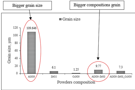
Figure 6: Comparison of average grain size
