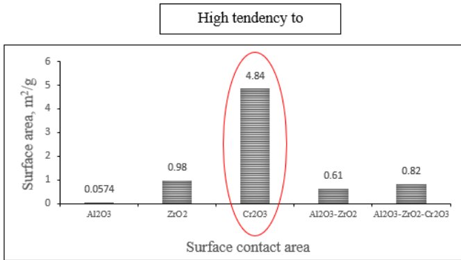
Figure 7: Comparison of surface contact area
