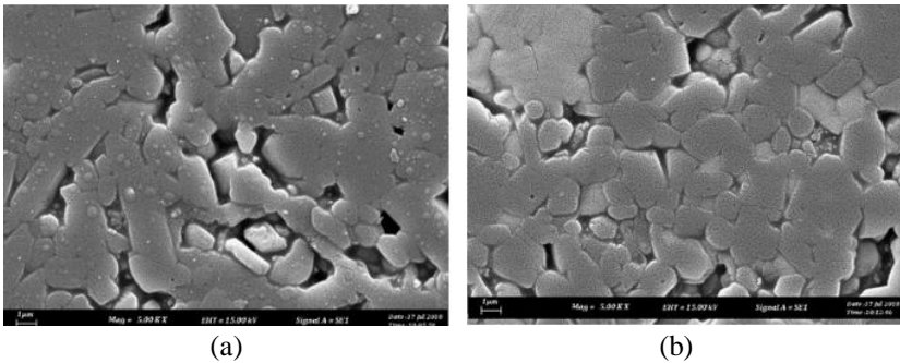
Figure 11: Cross-section comparison between (a) \text{Al}_2\text{O}_3 - \text{ZrO}_2 , and (b) \text{Al}_2\text{O}_3 - \text{ZrO}_2 - \text{Cr}_2\text{O}_3
