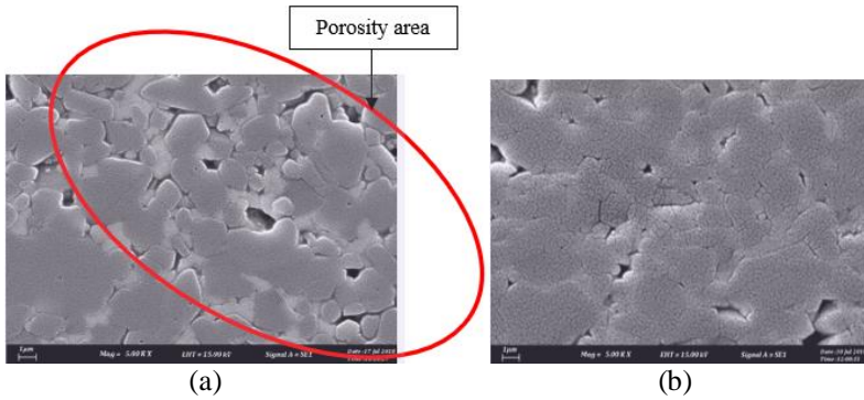
Figure 10: Surface comparison between (a) \text{Al}_2\text{O}_3 - \text{ZrO}_2 , and (b) \text{Al}_2\text{O}_3 - \text{ZrO}_2 - \text{Cr}_2\text{O}_3
