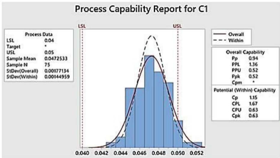
Figure 5: Process Capability Charts for the A7U43400 part;(a) before improvement, (b) after improvement
