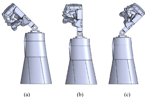
Fig. 2. Solidwork 3D Hand Design (a) Flexion Position, (b) Neutral Position, (c) Extension Position [70]
