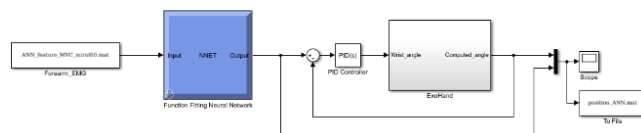
Fig. 10. Full system of exoskeleton hand for wrist movement with ANN and PID controller
