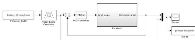
Fig. 11. Full system of exoskeleton hand for wrist movement with FL and PID controller [70].
