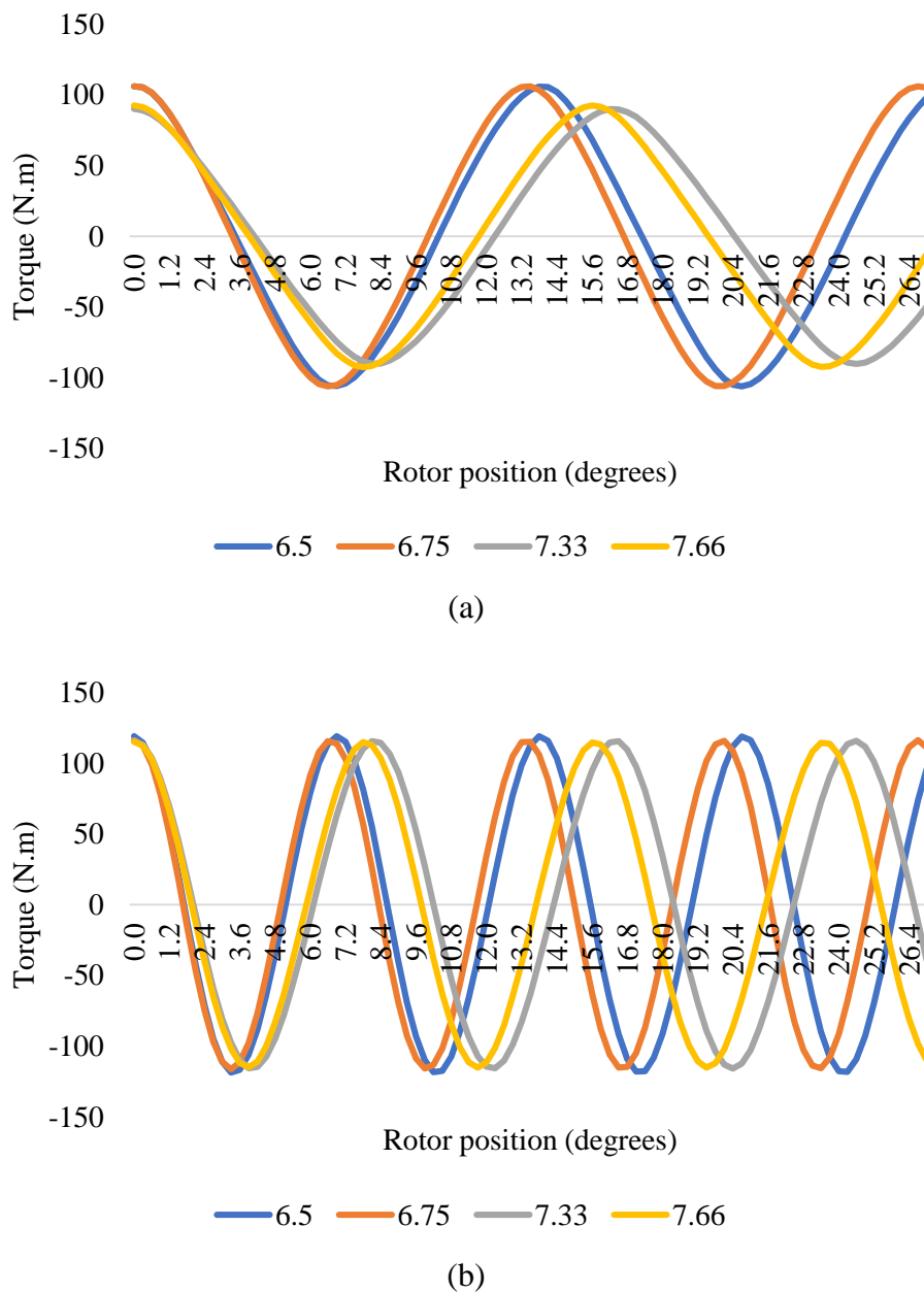
Fig. 7. Cogging torque in RPMG in the (a) 1 st combination and (b) 2 nd combination
