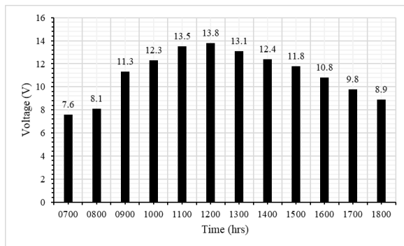
Fig. 9. Measured voltage from solar PV.
