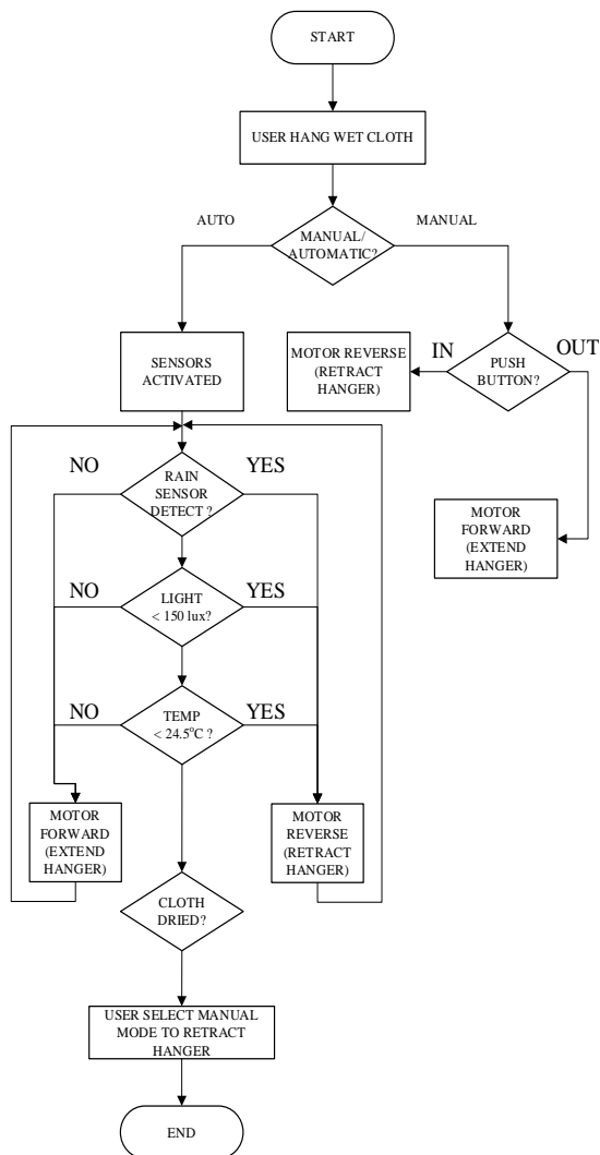
Fig. 9. Process flow.
