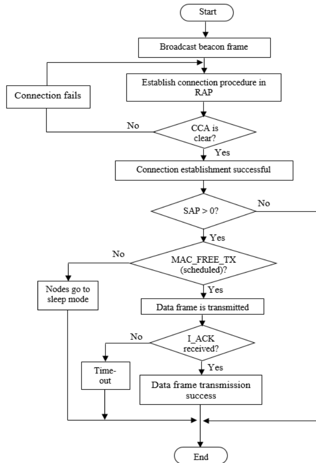
Figure 2. Flowchart of TDMA-MAC protocol
