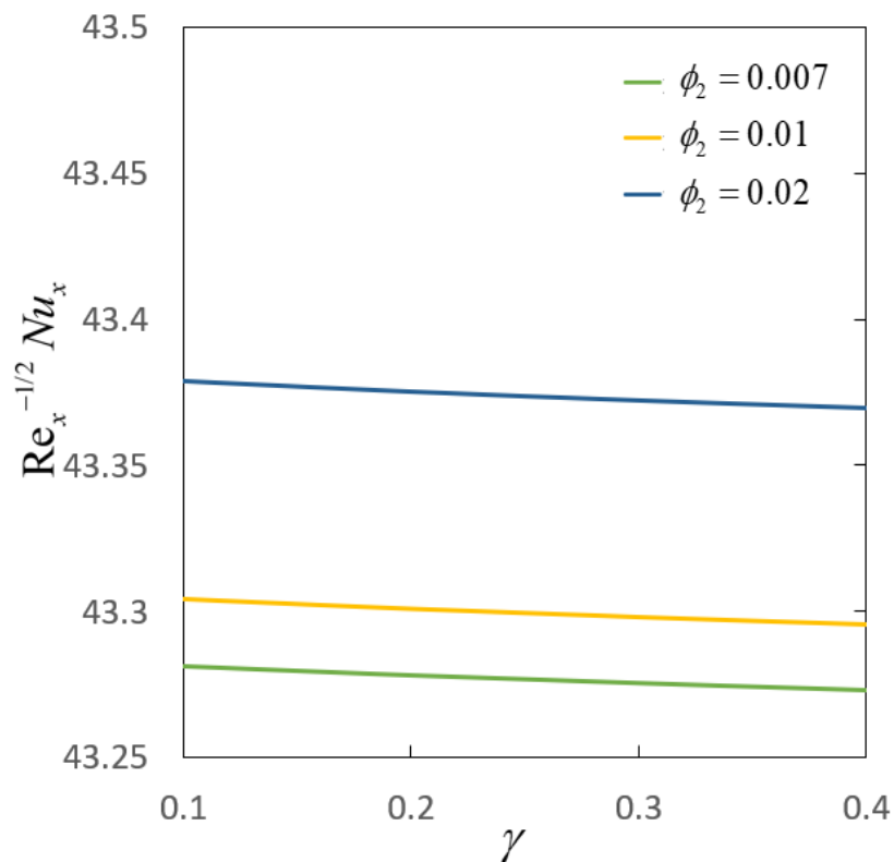
Fig. 9. Variation of Nusselt Number against Williamson parameter, \gamma for different values of \phi_2
