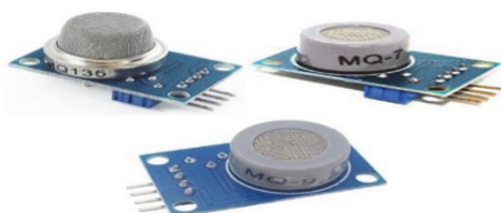
Fig.2. MQ135 gas sensor, MQ7 gas sensor, MQ9 gas sensor
