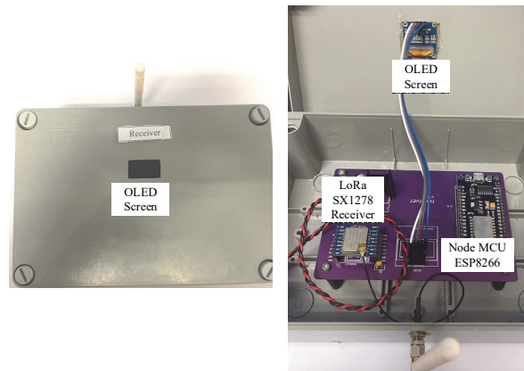
Fig.7. Receiver of Air Monitoring System
