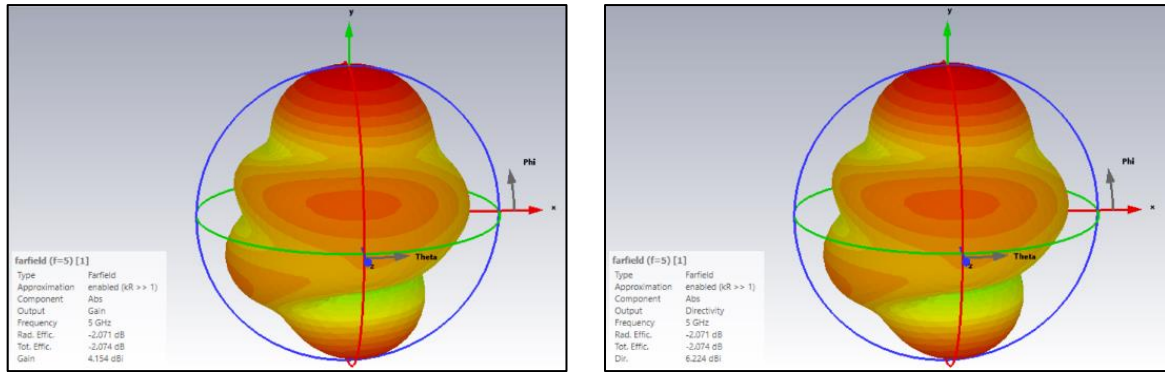
Figure 14: Radiation pattern of 5GHz frequency band
