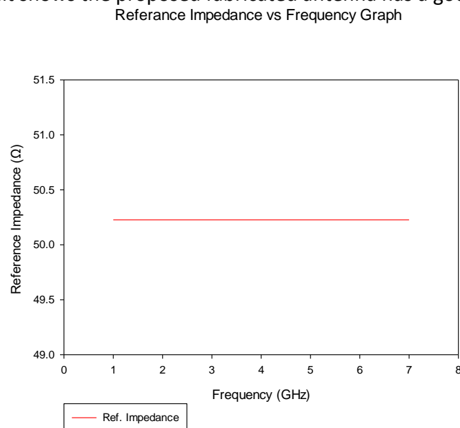
Figure 11: Reference impedance
