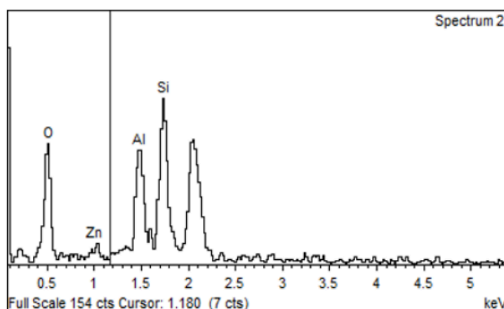
Fig. 4. EDX analysis
