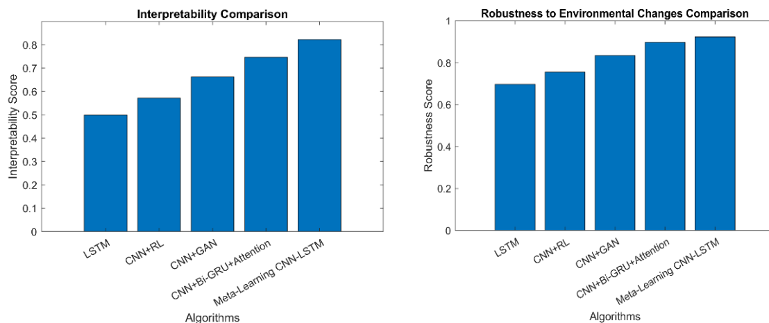
Figure 12. Comparative interpretability scores of algorithms in CSI-based HAR using Wi-Fi
