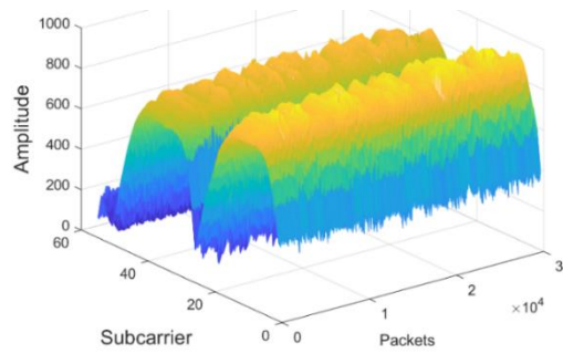
Figure 3. CSI amplitude for 2.4 GHz/20 MHz bandwidth
