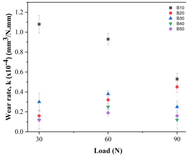
Figure 4: Wear rate of all the lubricant variants.
