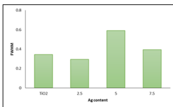
Fig. 2. FWHM of \text{Ag-TiO}_2 coated on unglazed tile
