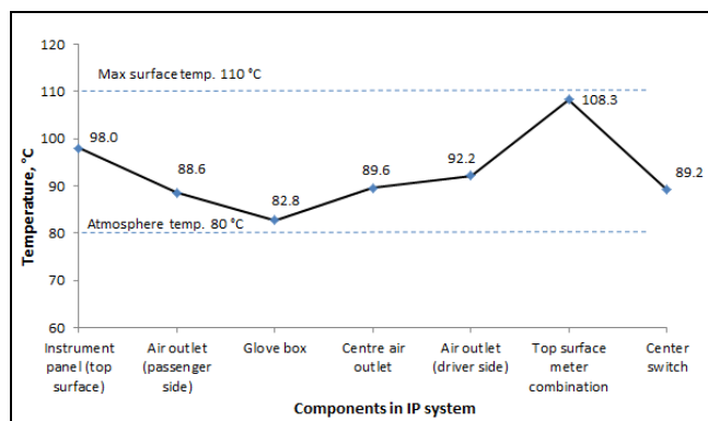
Figure 8. Maximum temperature achieved at component on IP system during infrared exposure heat cycle test.
