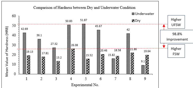
Figure 8: Comparison of hardness between dry and underwater conditions
