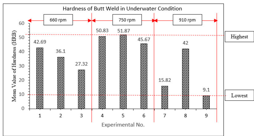
Figure 7: Result hardness of butt weld in underwater condition
