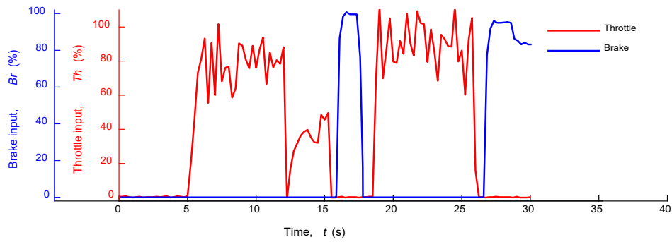
Figure 12. The evaluation of IWM-EV acceleration then braking performance on the level pavement at 15 km/h: (a) throttle and braking input, (b) vehicle dynamic characteristics and (c) electrical dynamic characteristics
