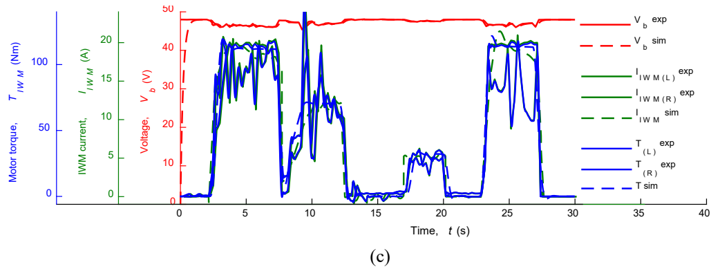
Figure 12. The evaluation of IWM-EV acceleration then braking performance on the level pavement at 15 km/h: (a) throttle and braking input, (b) vehicle dynamic characteristics and (c) electrical dynamic characteristics
