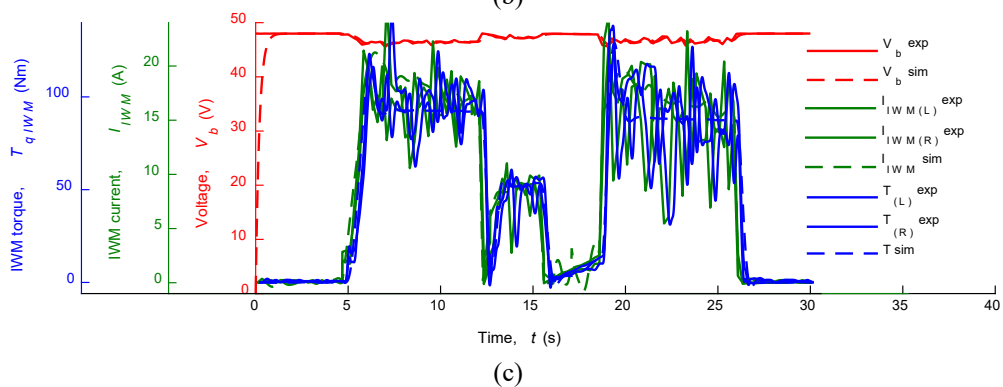
Figure 13. The evaluation of IWM-EV acceleration then braking performance on the level pavement at 20 km/h: (a) throttle and braking input; (b) vehicle dynamic characteristics; (c) electrical dynamic characteristics
