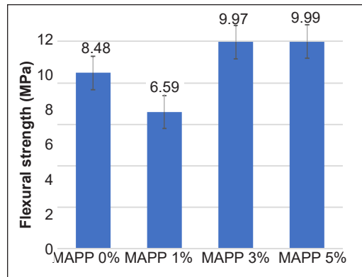
Figure 5. Flexural strength of r-WoPPc with MAPP
