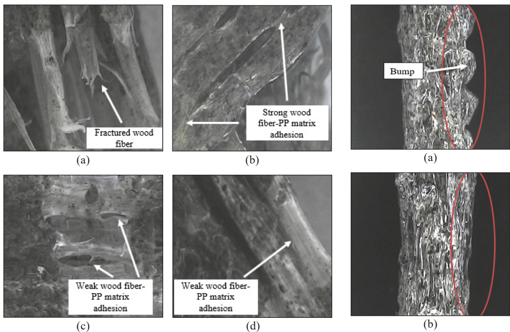
Figure 6. High precision micrograph with 10× magnification of r-WoPPc tensile fracture surface: (a) without MAPE; (b) 1 wt% MAPE; (c) 3 wt% MAPE; and (d) 5 wt% MAPE
