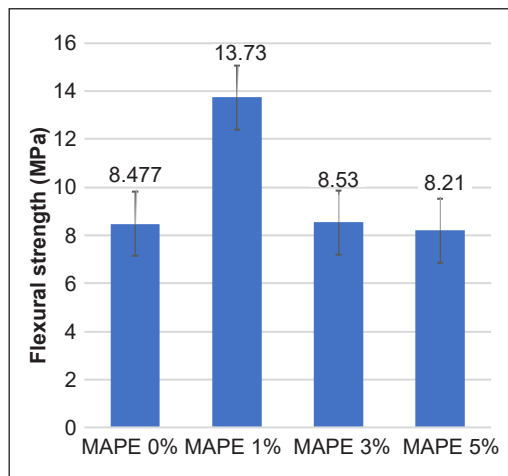
Figure 3 Flexural strength of r-WoPPc with MAPE
