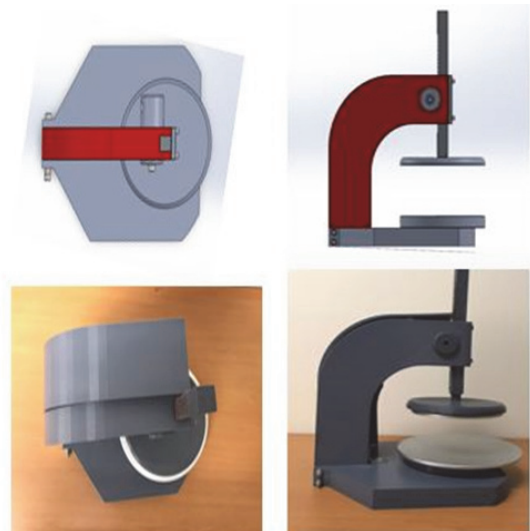
Fig.5. Prototype of an automatic press dough machine
