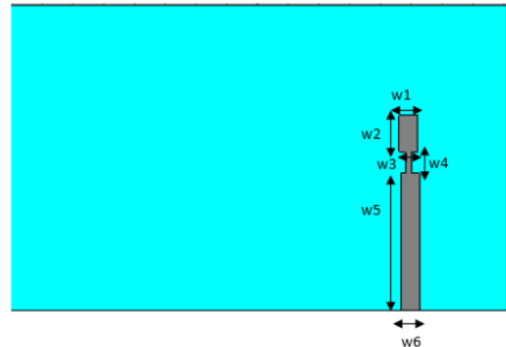
Figure 2 Drawing diagram of the proposed back view Vivaldi antenna
