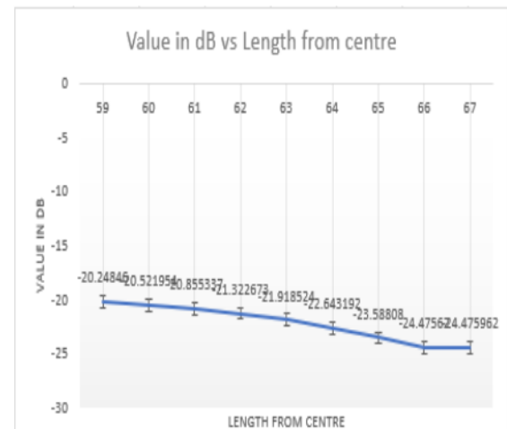
Figure 4 S-parameter value of dB vs length from center circle for S11 frequency at 3.5 GHz
