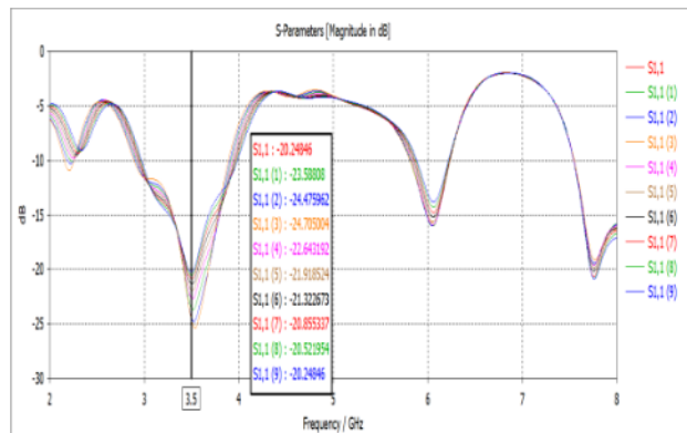
Figure 3 S-parameter analysis of length for PLA
