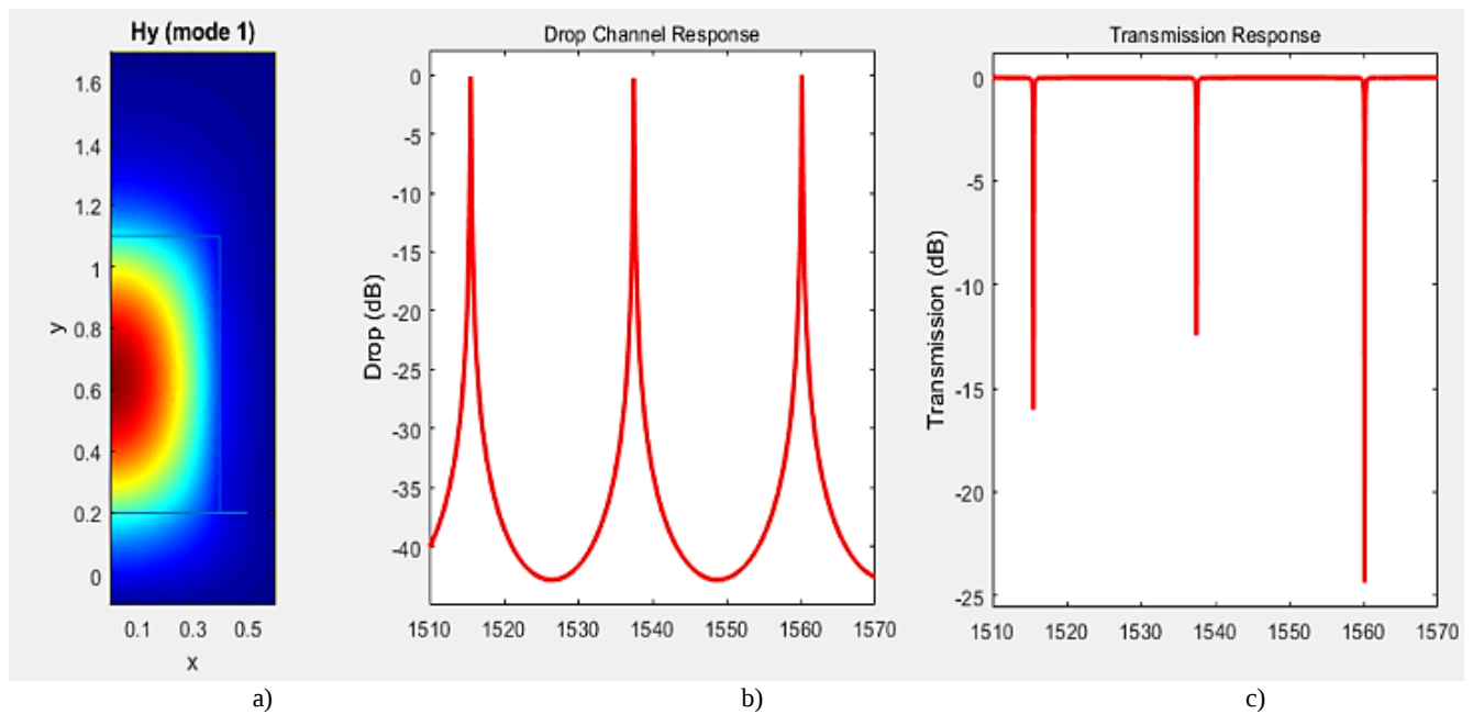
Fig. 3. (a) MRR fundamental mode profile (b) Optical MRR Response at drop port (c) Optical MRR Response at through port (color online)
