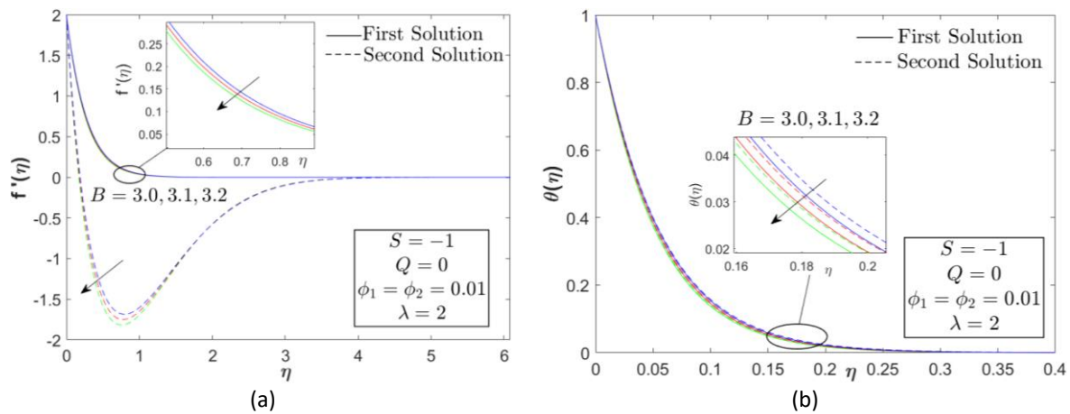
Fig. 7. (a) Velocity, and (b) temperature of Cu-Al 2 O 3 /H 2 O for the stretching case
