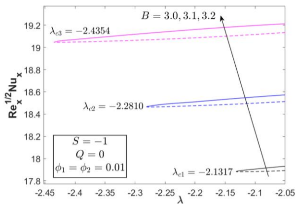
Fig. 3. Heat transfer rate over \lambda without heat generation ( Q = 0 ) and various suction parameter for graphene-alumina/water
