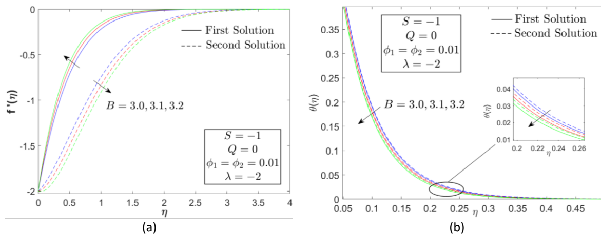
Fig. 6. (a) Velocity, and (b) temperature of Cu-Al 2 O 3 /H 2 O for the shrinking case
