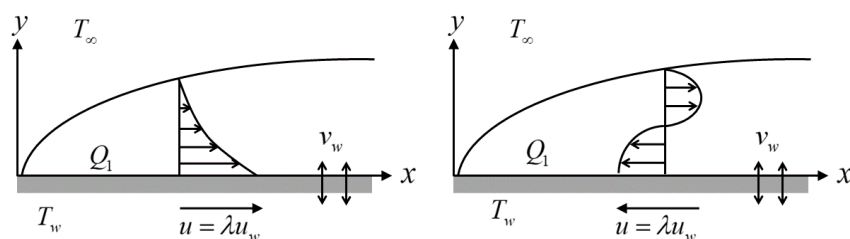
Fig. 1. Coordinate system of the physical problem for stretching (left) and shrinking (right) cases
