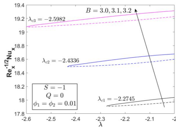
Fig. 5. Heat transfer rate over \lambda without heat generation ( Q=0 ) and various suction parameter for copper-alumina/water
