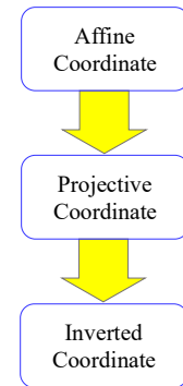
Fig. 5. Searching for an efficient count on arithmetic operations.
