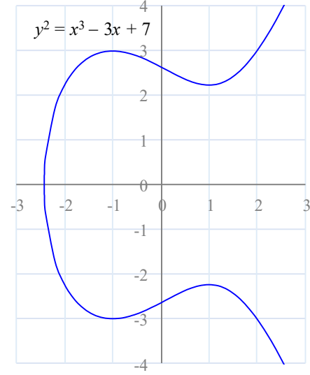
Fig. 2. A sample elliptic curve for b = 7 .
