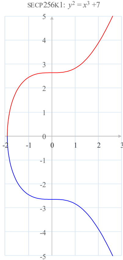
Fig. 1. A visual elliptic curve y^2 = x^3 + 7 .
