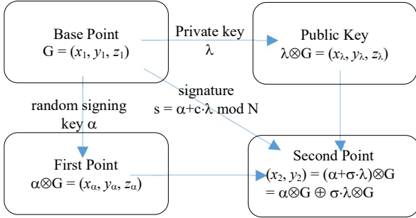
Fig. 6. Point projection in a basic digital signing and verification.
