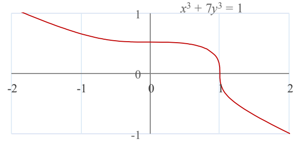
Fig. 4. A visual instance on a cubic Pell curve for c = 7 at the level z = 0 .
