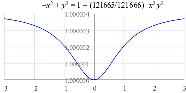
Fig. 3. An upper half of a twisted Edwards curve.
