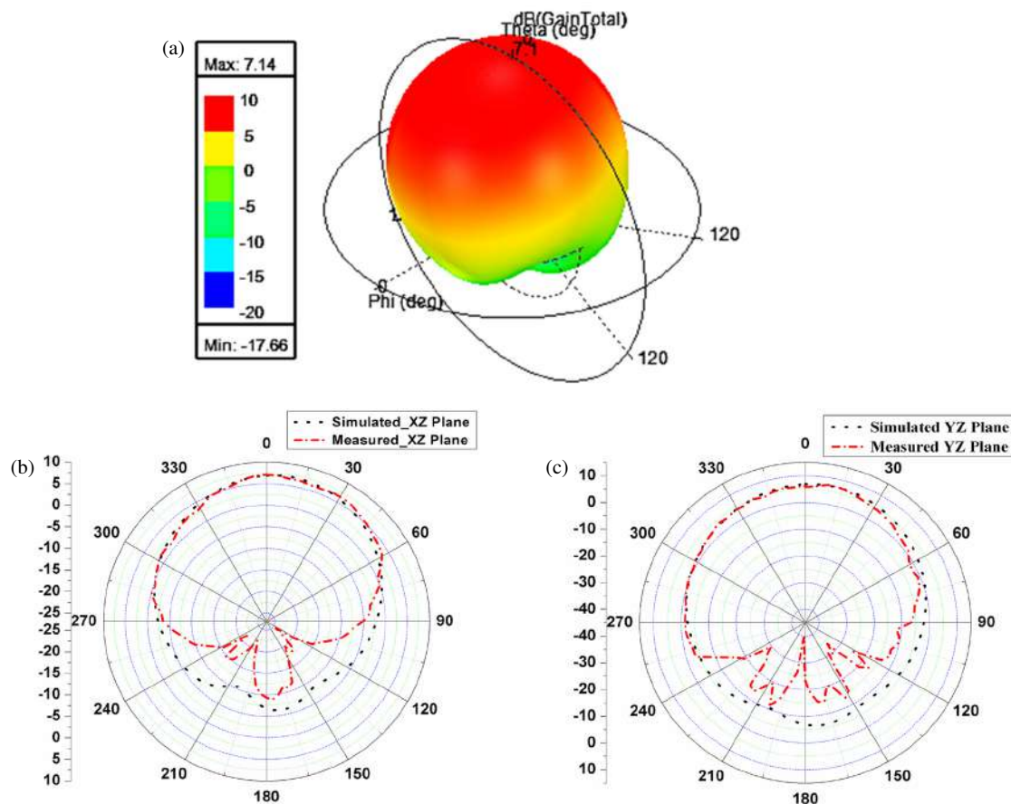
FIGURE 10. (a) 3D-gain plot. (b), (c) Measured vs. simulated radiation pattern ( XZ and YZ planes) plots at 5 GHz of the proposed design.
