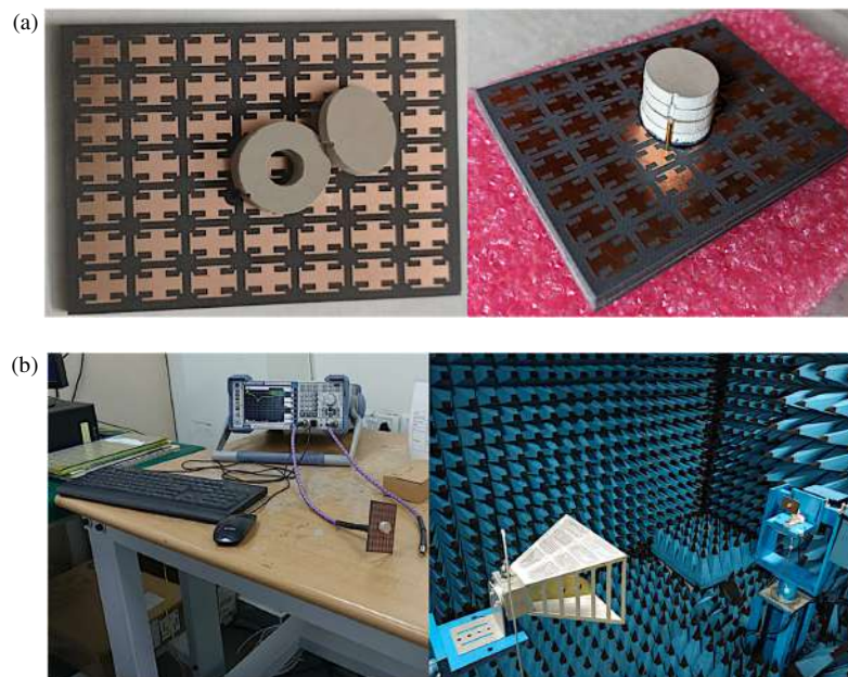
FIGURE 6. Fabricated HCDRA-2 (a) prototype before & after alignment and (b) its measurement setup in an anechoic chamber.
