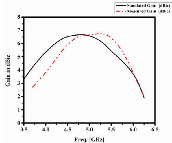
FIGURE 9. Gain vs. frequency plot.
