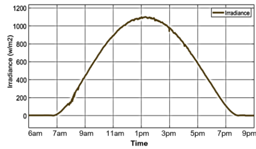
Figure 2. Nominal irradiance profile
