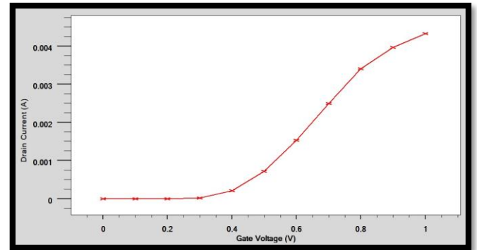
Figure 3. I_{DS} - V_{GS} characteristics of the NMOS device.
