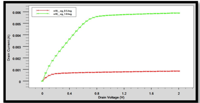
Figure 2. I_{DS} - V_{DS} characteristics of the NMOS device
