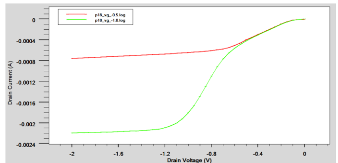
Figure 4. I_{DS} - V_{DS} characteristics of the PMOS device.
