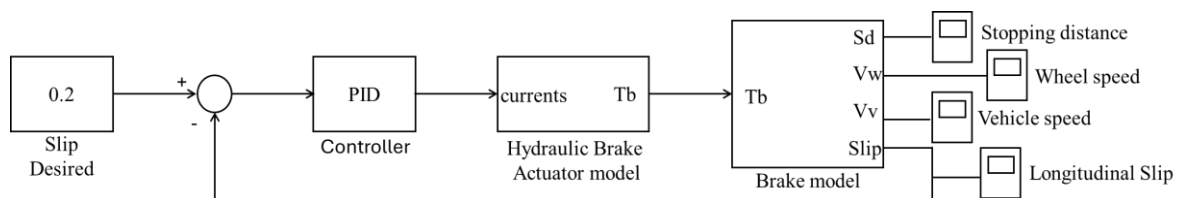
Figure 5. ABS control system
