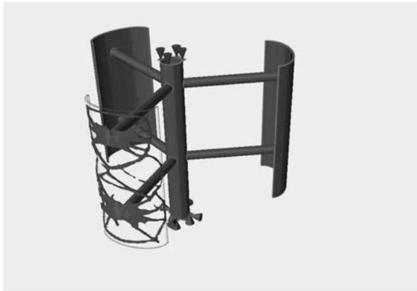
Fig. 4. Topology optimization
