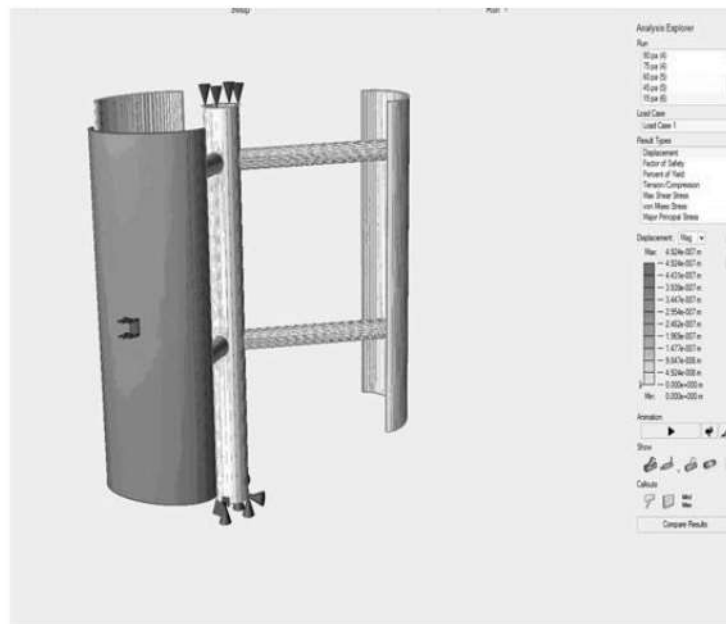
Fig. 2. Displacement Contour
