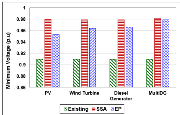
Figure 8 Comparison of minimum voltage for all cases
