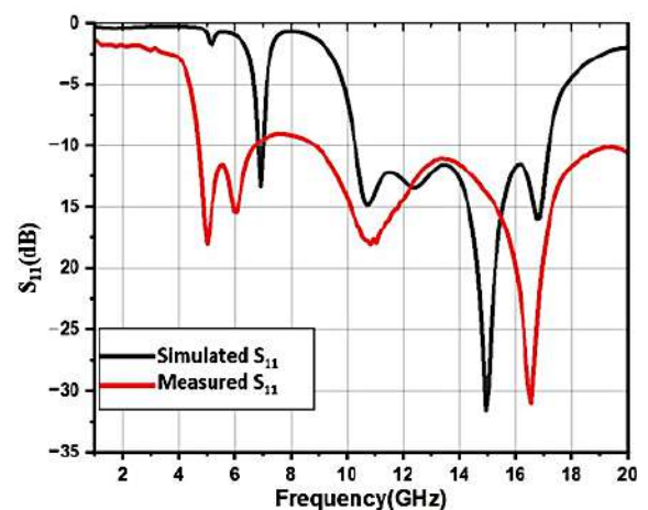
FIGURE 9. Simulated and measured reflection coefficients.
