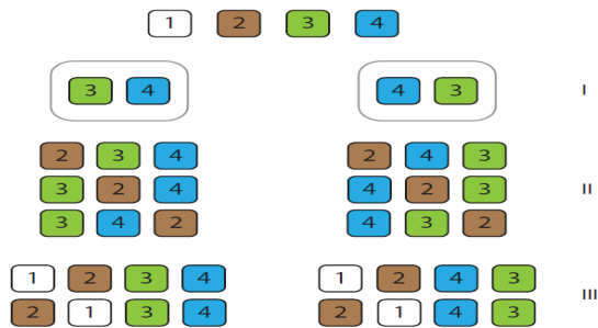
Figure 4: Permutation algorithm
