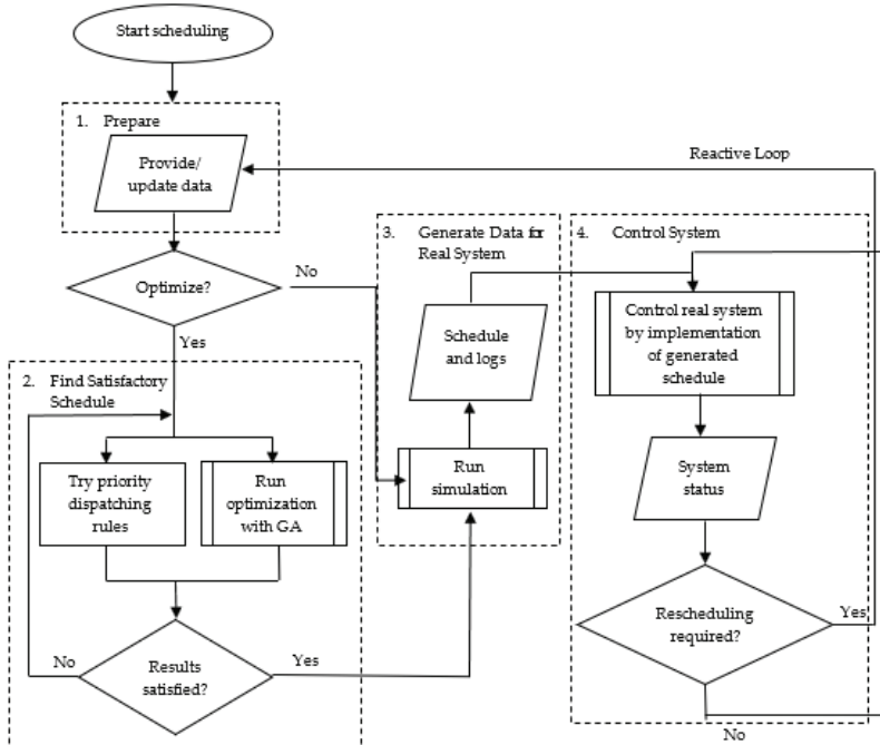
Figure 1: Scheduling procedure
