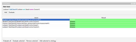
Figure 7: Axioms execution for Test 2 cardinality validation
