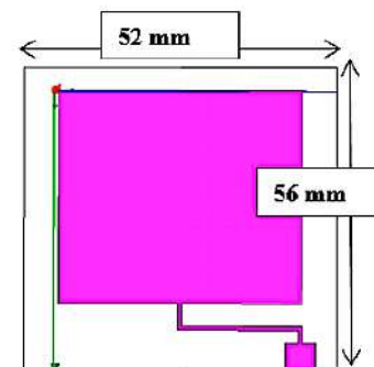
FIGURE 1. The design of the basic antenna element.
