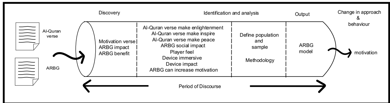
Fig. 4. Pipeline framework
