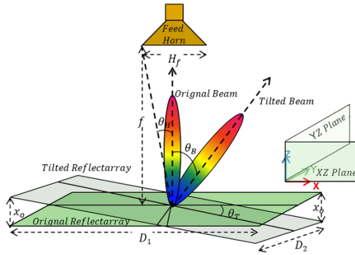
Figure 6. Schematic Diagram of beam-steering reflectarray antenna by mechanically rotating the array [37]
