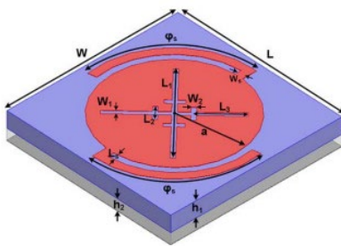
Figure 10 Proposed Unit Cell Element in [53]
