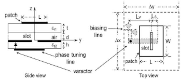
Figure 8. Reflectarray element [38] (a) Side view (b) Top view
