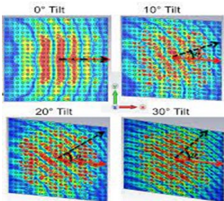
Figure 7 Different tilt angle effects on the phase of the surface current distribution [37]
