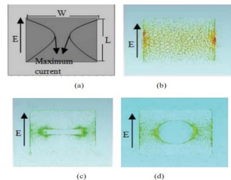
Figure 9 Proposed Reflectarray Design [39] (a) a unit cell showing E-field with maximum surface current (b) Surface current without slot (c) Surface current with rectangular slot (d) Surface current with circular slot.
