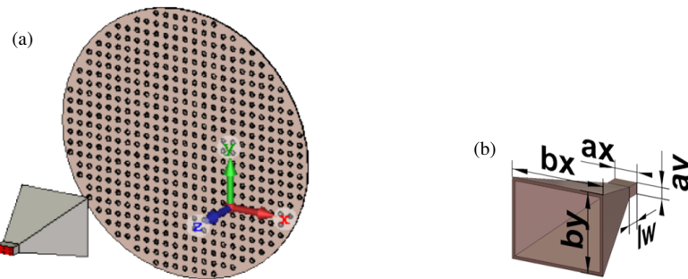
FIGURE 6. (a) Reflectarray design with feed antenna and (b) feed antenna design (with dimensions ax = 168 \mu\text{m} , ay = 47 \mu\text{m} , bx = 881 \mu\text{m} , by = 715 \mu\text{m} , lw = 136 \mu\text{m} ).
