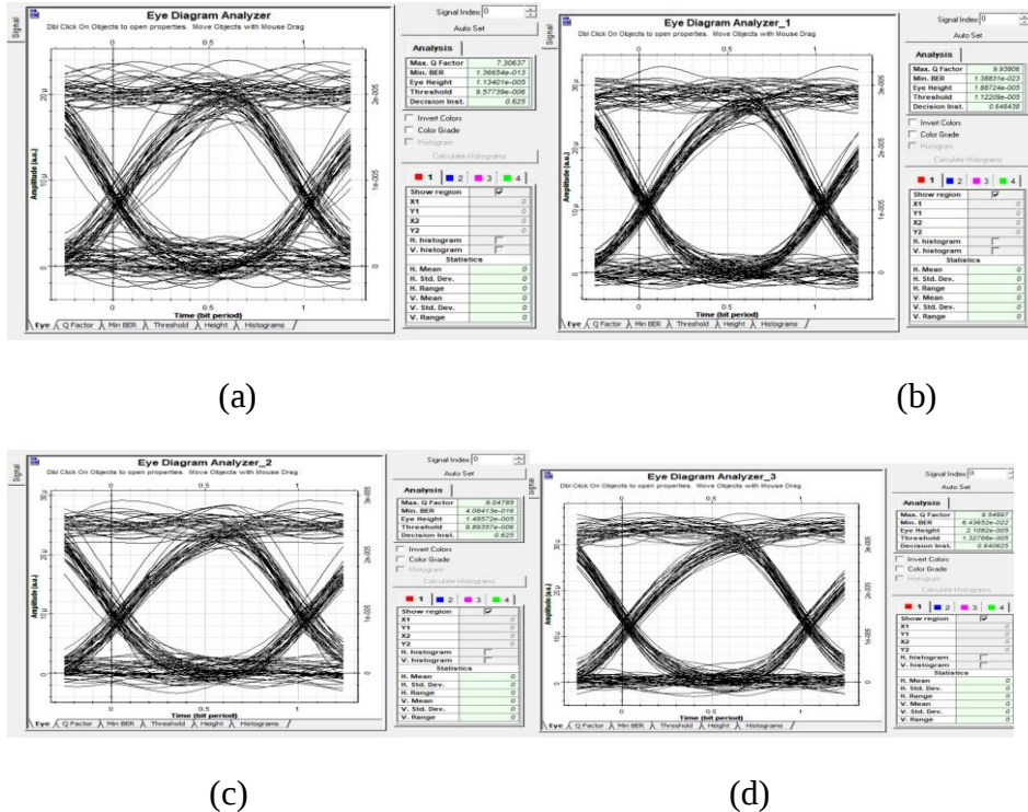
Figure 3: eye diagrams obtained from each channel (a) 193.1 THz, (b) 193.2 THz, (c) 193.3 THz, (4) 193.4 THz
