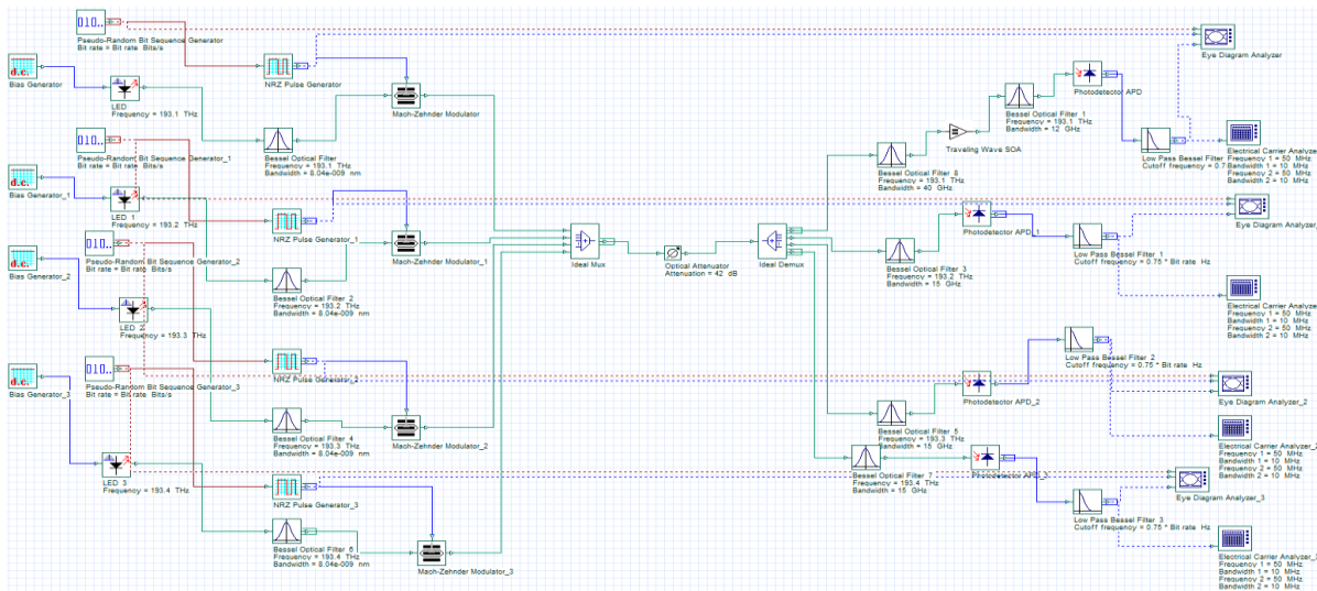
Figure 2: WDM set-up used with SOA enhancement
