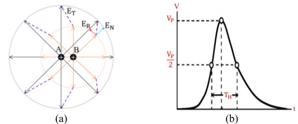
FIGURE 2. EM radiation of partial discharge: (a) charge acceleration (b) voltage waveform.
