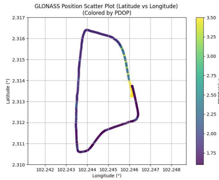
Fig. 18 Position scatter plot (latitude vs longitude) of GLONASS configuration conducted in a kinematic manner
