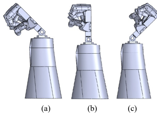
Fig. 1: Solidwork 3D Hand Design (a) Flexion Position, (b) Neutral Position, (c) Extension Position.
