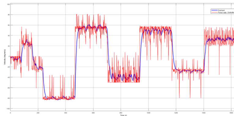
Fig. 15: Fuzzy Logic and PID controller for Estimated wrist desired velocity of Exoskeleton hand using ECRL muscle.
