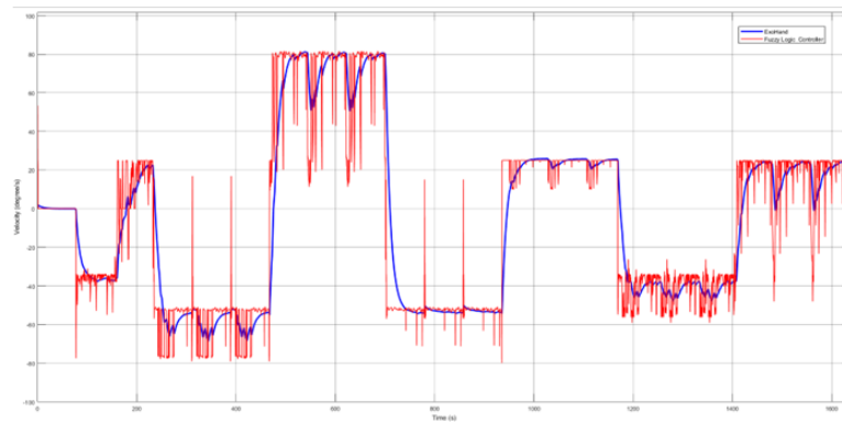
Fig. 14: Fuzzy Logic and PID controller for Estimated wrist desired velocity of Exoskeleton hand using FCR muscle.
