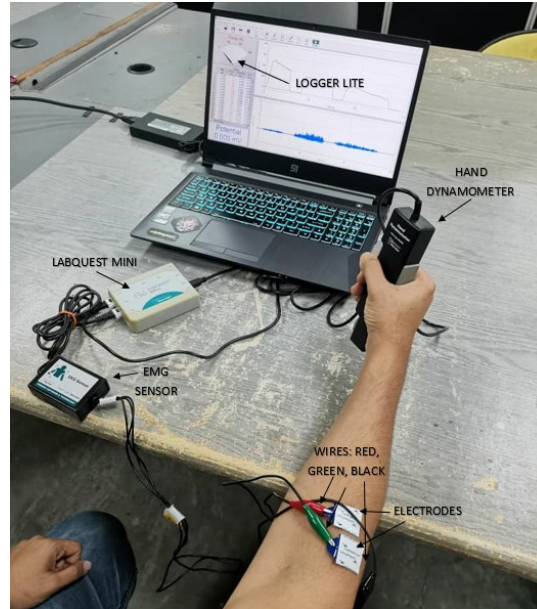
Fig. 2: Experimental set-up.
