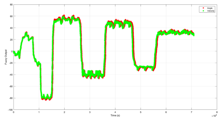
Fig. 8: ECRL muscle response from fuzzy logic output.
