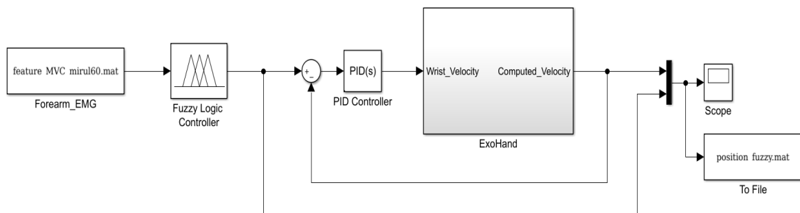
Fig. 13: Full system of exoskeleton hand for wrist movement with FL and PID controller.
