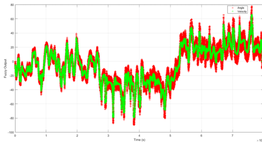
Fig. 11: Fuzzy output for 20% MVC.
