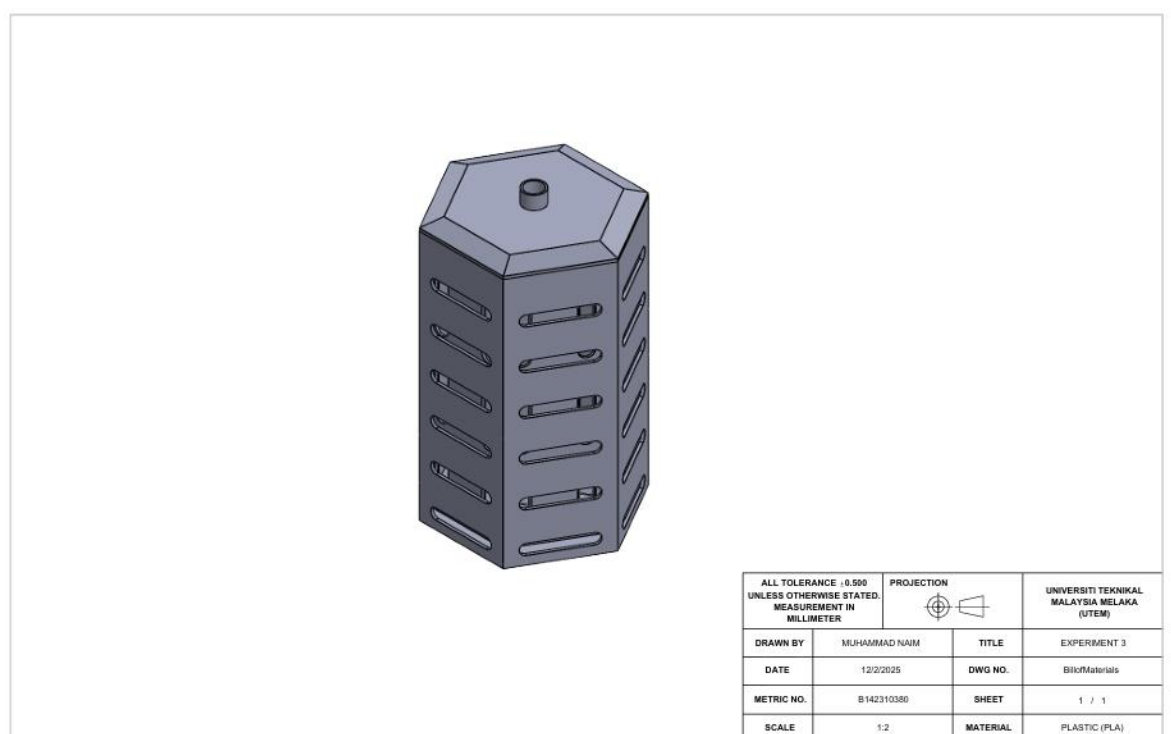
Figure 4. DHS Casing Design
