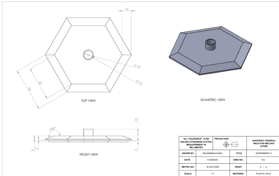
Figure 5. DHS Casing Design
