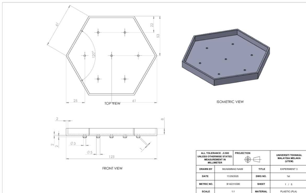
Figure 2. DHS Casing Design
