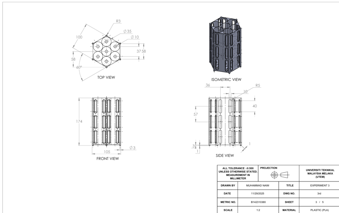
Figure 1. DHS Casing Design
