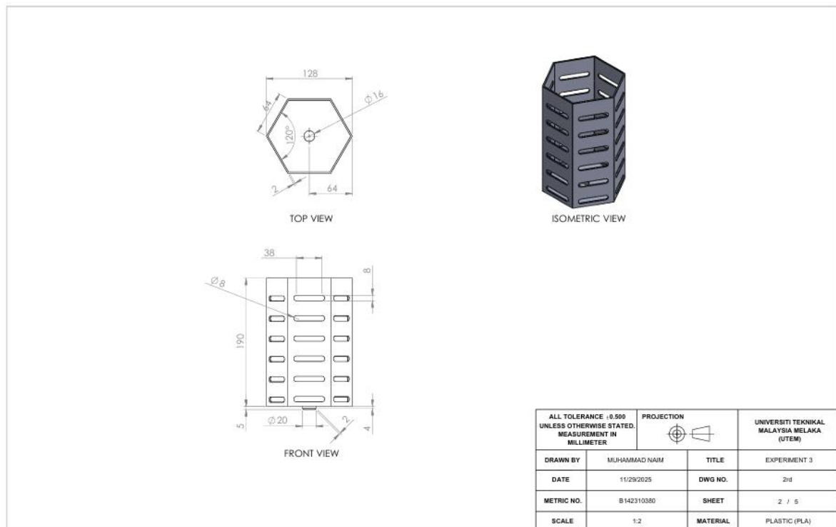
Figure 3. DHS Casing Design
