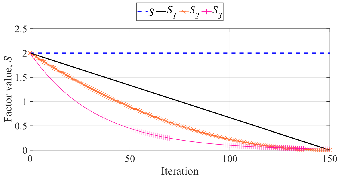
Fig. 1. Fixed S factor and proposed dynamic S_1 , S_2 , and S_3 factor values.
