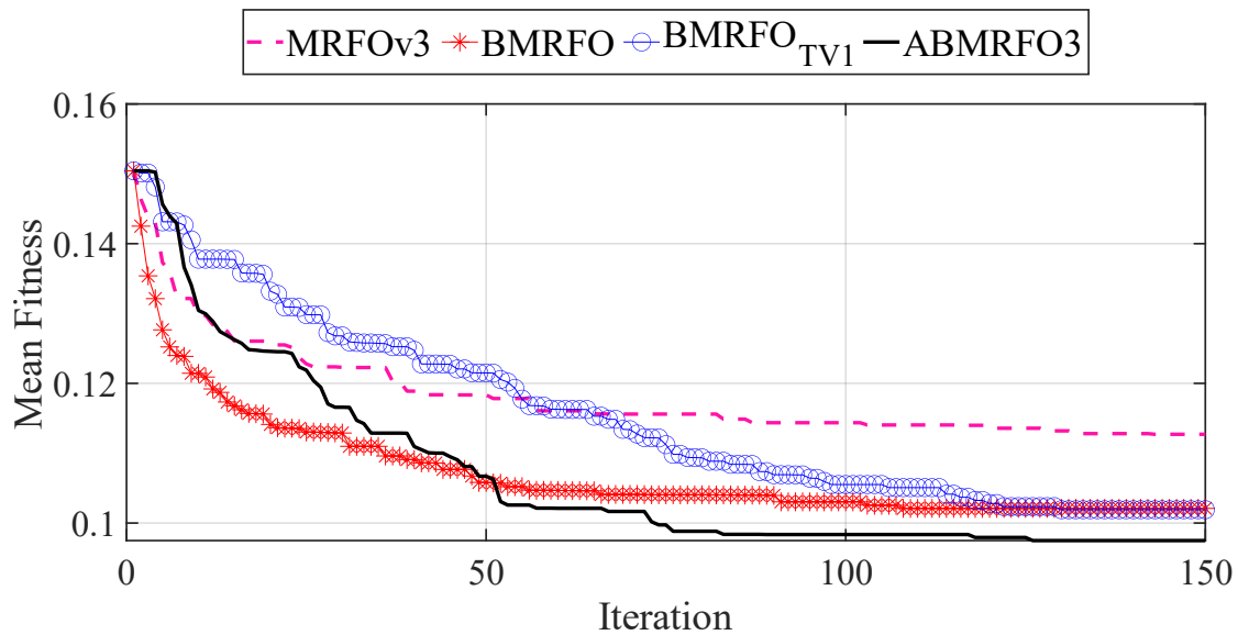
Fig. 3. Convergence graph of the proposed ABMRFO3 and existing BMRFO variants.
