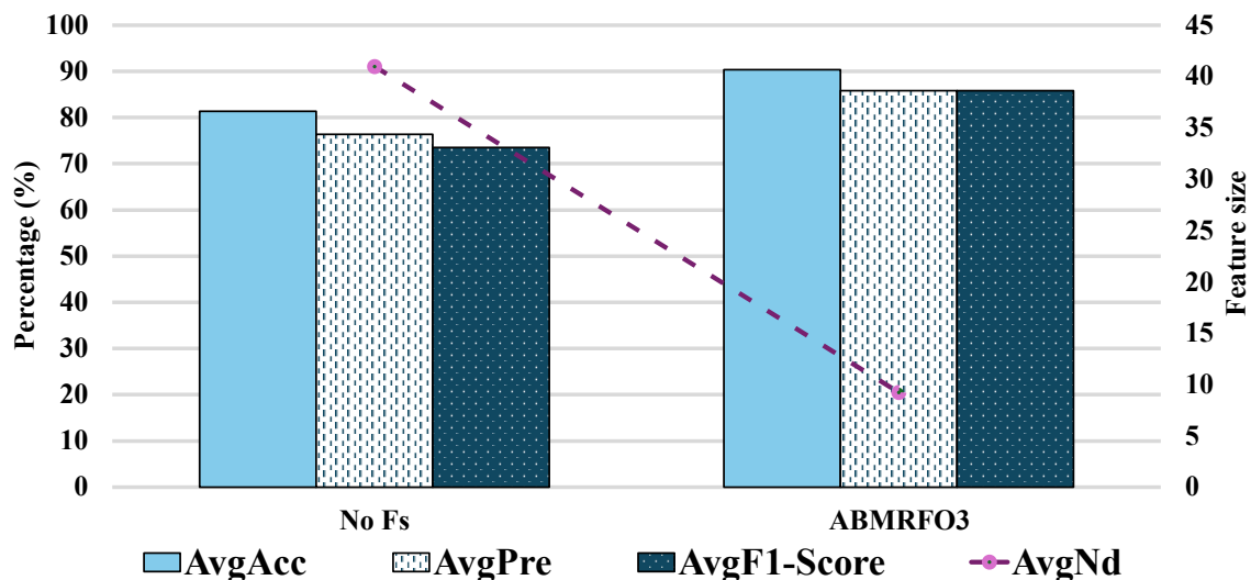
Fig. 4. Comparison of classification performance with and without feature selection.
