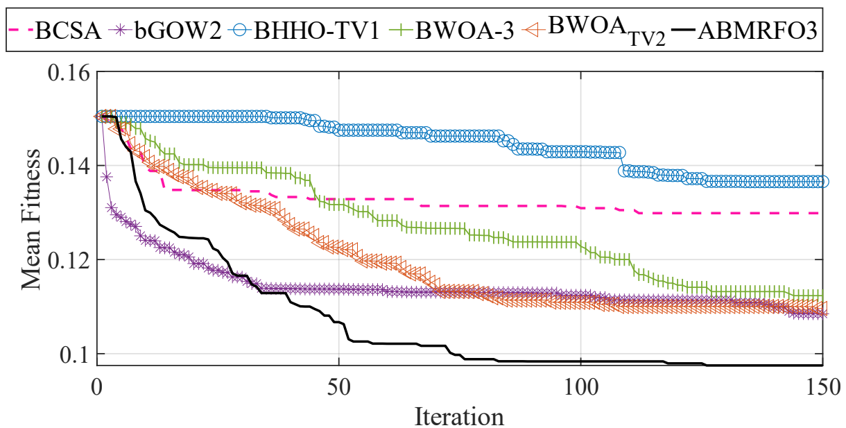
Fig. 5. Convergence curves of the proposed ABMRFO3 with other state-of-the-art SI algorithms.
