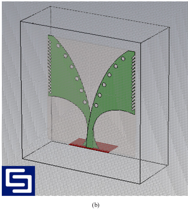
Fig. 1 SAVA antenna layout, (a) Geometric layout, (b) CST layout
