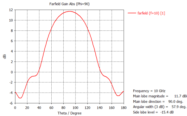
Fig. 5 Simulated gain of SAVA in H-plane at 10 GHz
