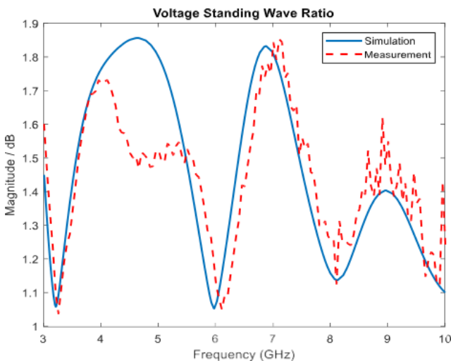
Fig. 8 Measured and simulated VSWR
