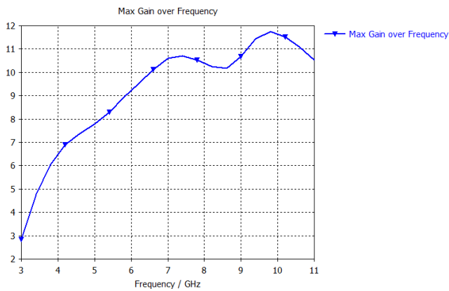
Fig. 4 Simulated gain of SAVA over UWB band
