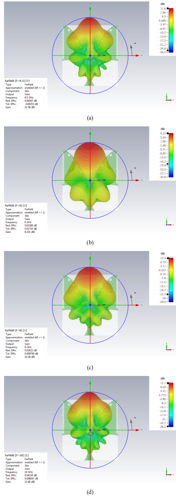
Fig. 3 Three-dimensional far-field radiation pattern of SAVA, (a) 4 GHz, (b) 6 GHz, (c) 8 GHz, (d) 10 GHz
