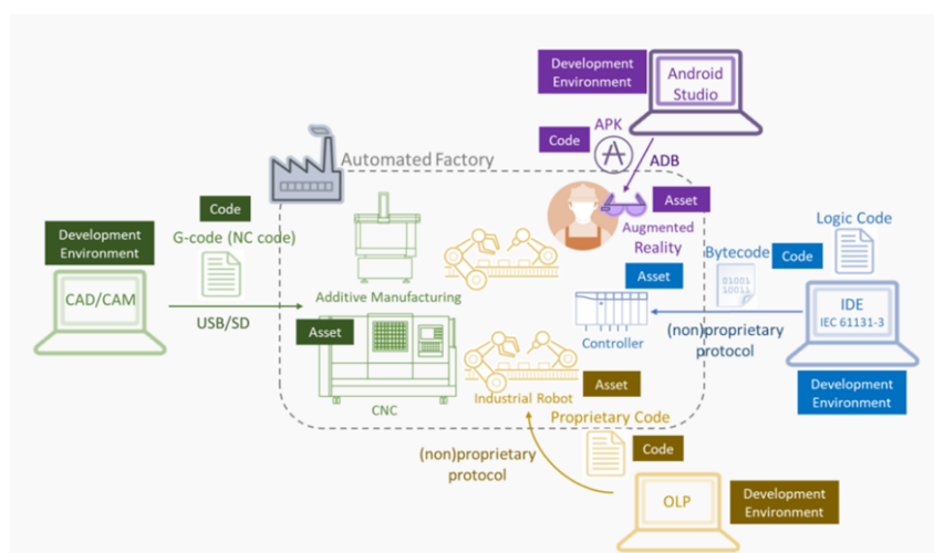
Figure 1 Schematic of the integrated system architecture in a factory with lights out (Adapted from TXOne Networks, 2023)
